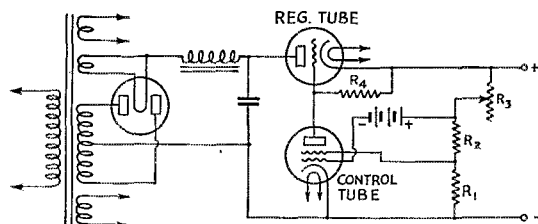
FIG. 4—ESSENTIAL CIRCUIT OF THE W.E. VOLTAGE-REGULATED POWER SUPPLY
